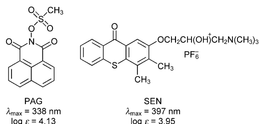
Scheme 2. Molecular formulae of the photoacid generator (PAG) used to switch the protonation state of the green Bodipy dye and of the oxothioxanthene (SEN) sensitizer employed as UV activator. The spectral absorption properties are given in each case and spectra are shown in the Supporting Information.
